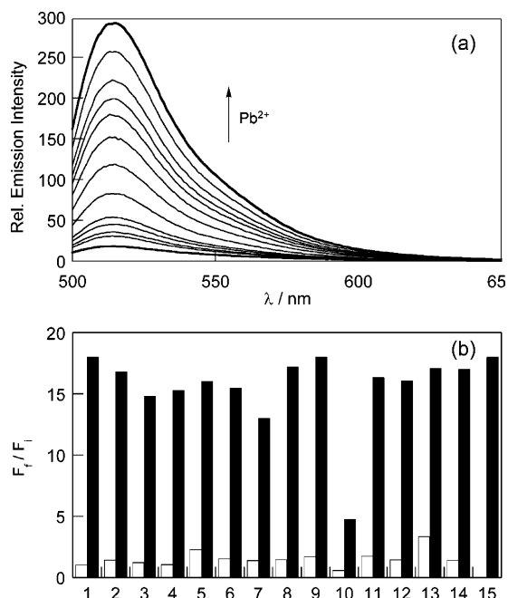
Figure 1. (a) Fluorescence response of 5 \mu\text{M} LF1 to \text{Pb}^{2+} . Spectra shown are for \text{Pb}^{2+} concentrations of 0, 1, 2, 3, 4, 5, 10, 15, 20, 25, 35, 50, and 75 \mu\text{M} . Spectra were acquired in 20 mM HEPES, pH 7, with excitation at 490 nm. (b) Fluorescence responses of 5 \mu\text{M} LF1 to various metal ions. Bars represent the final integrated fluorescence response ( F_t ) over the initial integrated emission ( F_i ). Spectra were acquired in 20 mM HEPES, pH 7. White bars represent the addition of an excess of the appropriate metal ion (2 mM for \text{Li}^+ , \text{Na}^+ , \text{K}^+ , \text{Mg}^{2+} , and \text{Ca}^{2+} , 75 \mu\text{M} for all other cations except entry 11) to a 5 \mu\text{M} solution of LF1. Black bars represent the addition of 75 \mu\text{M} \text{Pb}^{2+} to the solution. Excitation was provided at 490 nm, and the emission was integrated over 500–650 nm. 1, \text{Li}^+ ; 2, \text{Na}^+ ; 3, \text{K}^+ ; 4, \text{Mg}^{2+} ; 5, \text{Ca}^{2+} ; 6, \text{Mn}^{2+} ; 7, \text{Fe}^{2+} ; 8, \text{Co}^{2+} ; 9, \text{Ni}^{2+} ; 10, \text{Cu}^{2+} ; 11, \text{Cu}^{2+} , 25 \mu\text{M} ; 12, \text{Zn}^{2+} ; 13, \text{Cd}^{2+} ; 14, \text{Hg}^{2+} ; 15, \text{Pb}^{2+} .
